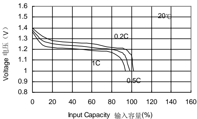
0.2C/0.5C/1C Rate Discharge Curves
