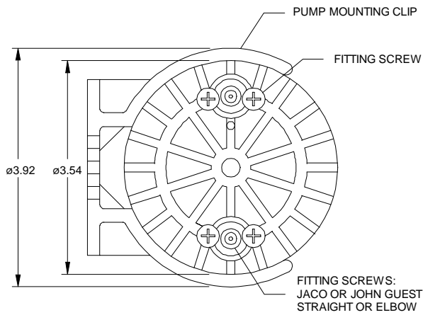
FIGURE 1. PERMEATE PUMP DIMENSIONS
